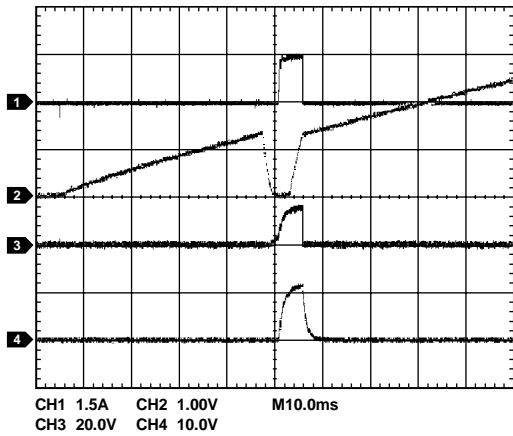
Figure 45. Overcurrent Condition at Startup (ADM1178-1 Model) (CH1 = I_{LOAD} , CH2 = V_{TIMER} , CH3 = V_{GATE} , CH4 = V_{OUT} )
