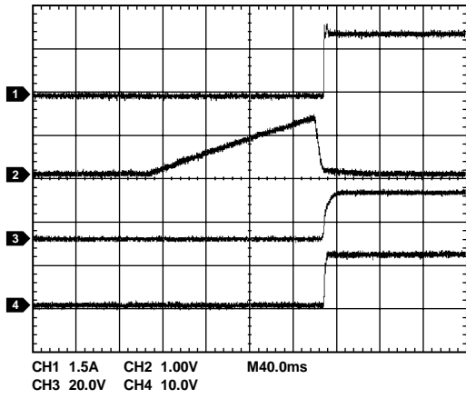
Figure 44. Inrush Current Control into 220 \mu F Load (CH1 = I_{LOAD} , CH2 = V_{TIMER} , CH3 = V_{GATE} , CH4 = V_{OUT} )
