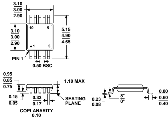
COMPLIANT TO JEDEC STANDARDS MO-187-BA Figure 51. 10-Lead Mini Small Outline Package [MSOP] (RM-10) Dimensions shown in millimeters
