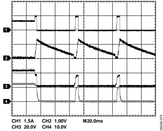
Figure 48. Overcurrent Condition During Operation (ADM1178-2 Model) (CH1 = I_{LOAD} , CH2 = V_{TIMER} , CH3 = V_{GATE} , CH4 = V_{OUT} )
