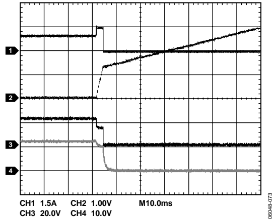
Figure 47. Overcurrent Condition During Operation (ADM1178-1 Model) (CH1 = I_{LOAD} , CH2 = V_{TIMER} , CH3 = V_{GATE} , CH4 = V_{OUT} )
