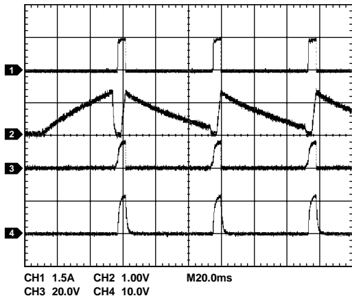
Figure 46. Overcurrent Condition at Startup (ADM1178-2 Model) (CH1 = I_{LOAD} , CH2 = V_{TIMER} , CH3 = V_{GATE} , CH4 = V_{OUT} )
