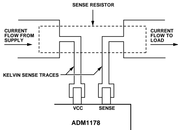
Figure 50. Kelvin Sense Connections
